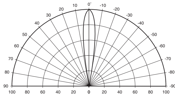
Fig. 5 Radiation Pattern
